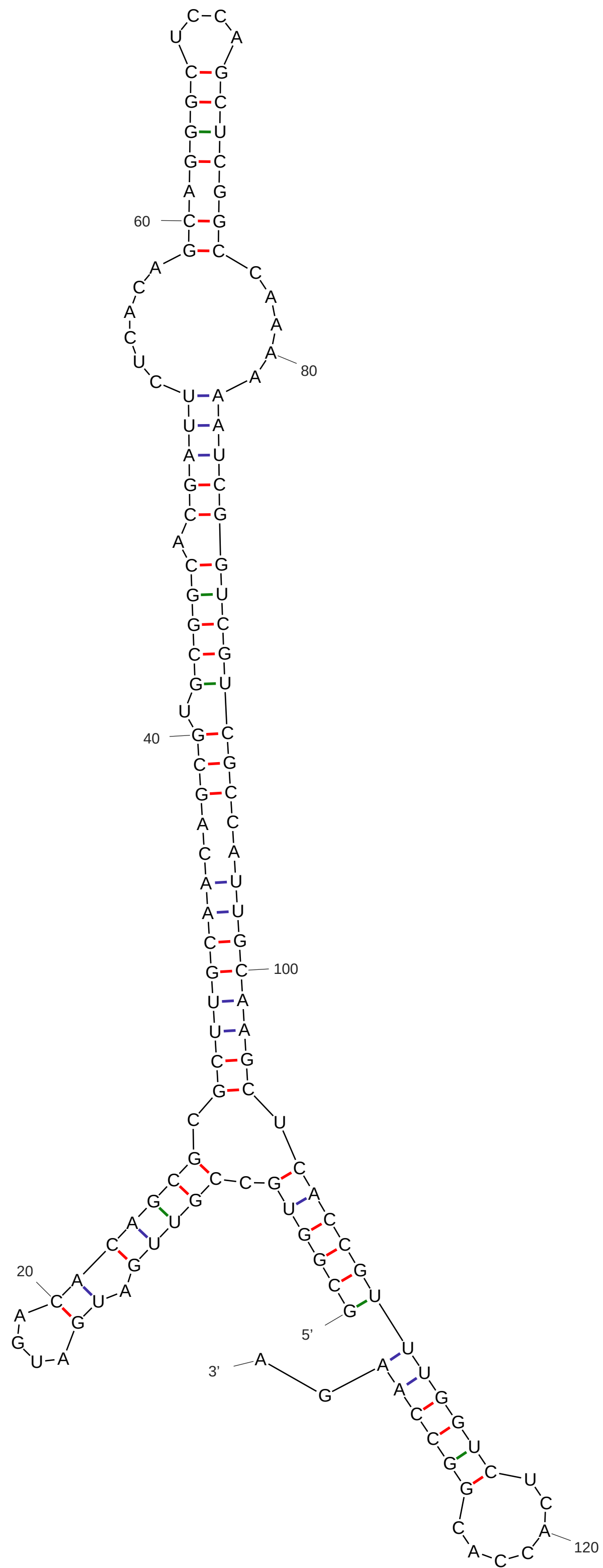
dG = -52.70 [Initially -53.30] dme-mir-4987 MI0017773
